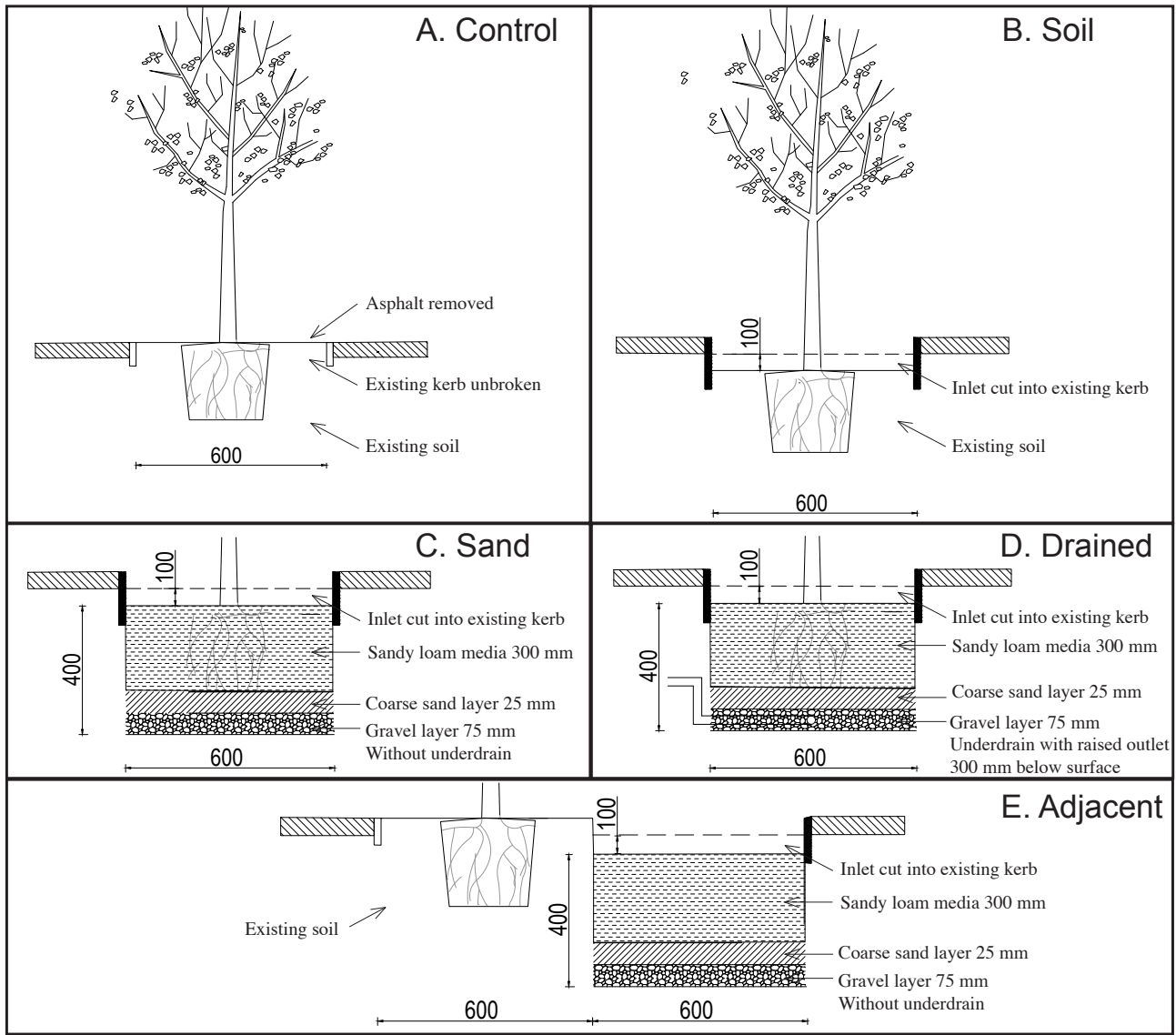
Figure 1: Cross section drawings of (A) Control, (B) Soil, (C) Sand, (D) Drained, (E) Adjacent treatments showing differences in inlet locations, soil/substrate types, drainage connections and tree locations.
